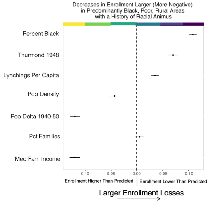
Figure 7. Geographic distribution and correlates of differential enrollment losses. Correlates are standardized within states. Enrollment losses are defined as the difference between predicted enrollment and observed enrollment. Enrollment is predicted using not-yet-treated and never-treated observations, as described in Section 6.1. The x-axis indicates the change in estimated treatment effect associated with a one standard deviation change in the correlate. For example, a one standard deviation increase in Percent Black is associated with an additional .1 log point loss in enrollment due to segregation academies.
