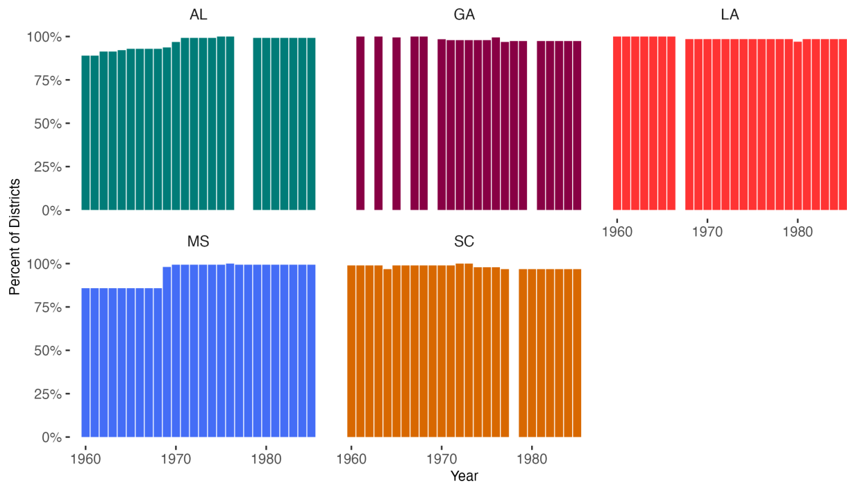
Figure A.2. Graph of non missing observations for enrollment.
