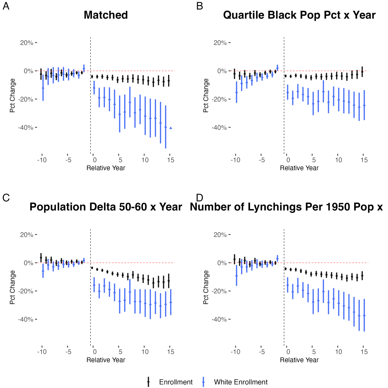
Figure A.3. Event studies showing results from Table 2.
