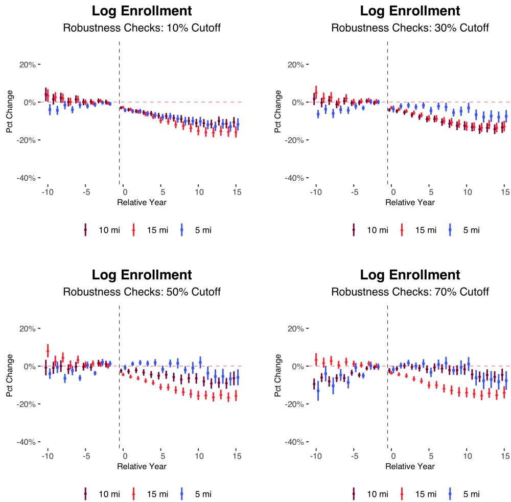
Figure A.5. Robustness checks. 10%, 30%, and 50% yield similar results. The more restrictive criteria of shrinking the radius of the catchment area to 5 miles or requiring 70% of the school district's area to be within the catchment area reduces the number of treated counties such that results become noisy and subject to pre-trends.
