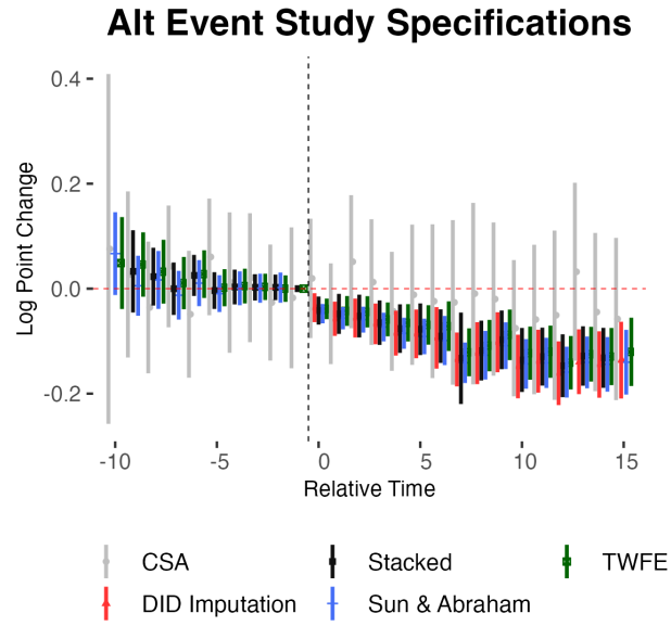
Figure A.4. Results using alternate TWFE specifications. CSA refers to Callaway and Sant'Anna 2020. Points represent the average of the estimates; bars represent the 95% confidence intervals of these estimates.
