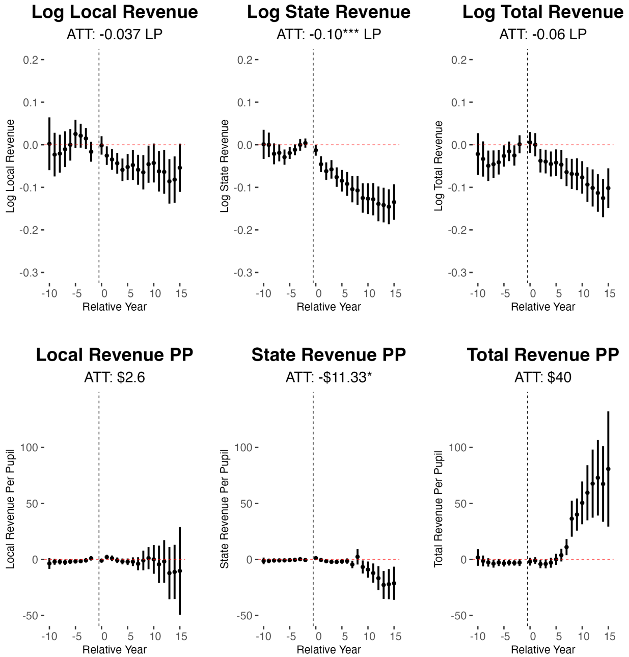
Figure 8. The impact of segregation academies on funding outcomes. Georgia is omitted because it only has funding data available for 11 of the 25 years of interest, and no data is available after 1976. Panels A-D correspond to columns (1)-(4) of Table 8, respectively. Control means for local funding per pupil and total funding per pupil are $161 and $604, respectively. 95 percent confidence intervals are represented by vertical bars.
